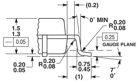
VIEW AA
