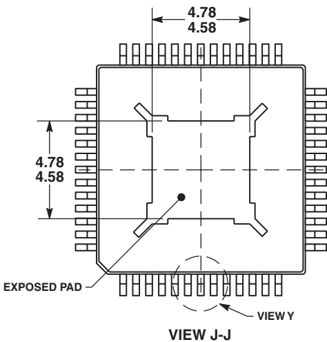
VIEW J-J
